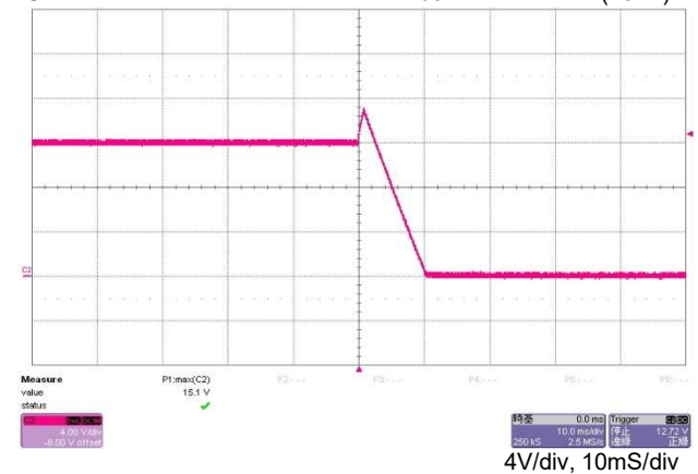
OVP 60% of rated load(264V)
