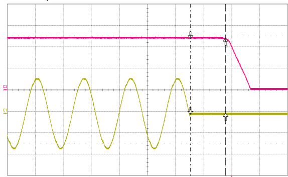
Hold-up time rated load
