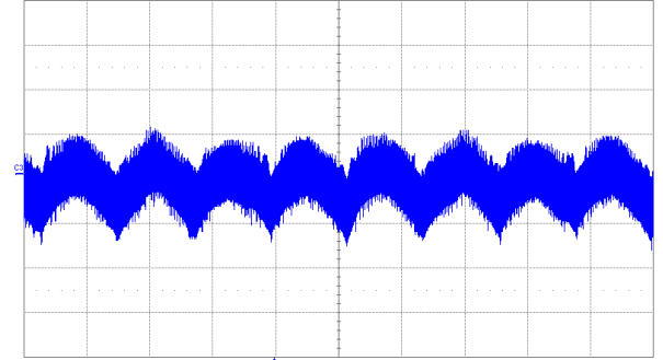
Line frequency ripple rated load
